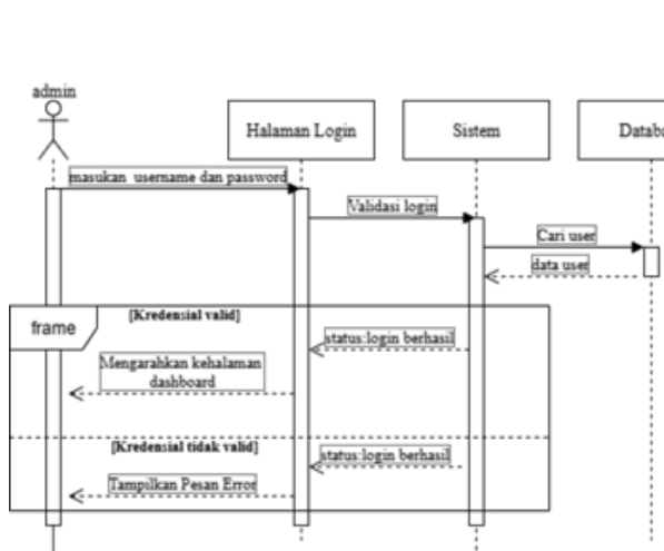
Figure 6. Login Sequence Diagram
