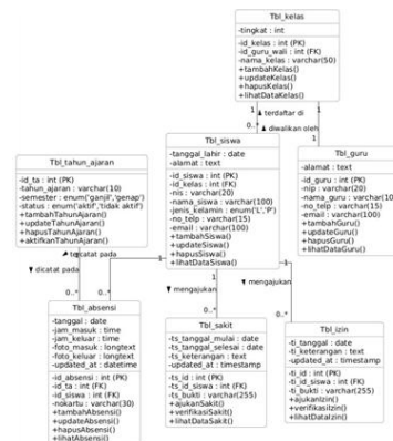
Figure 9. Class Diagram
