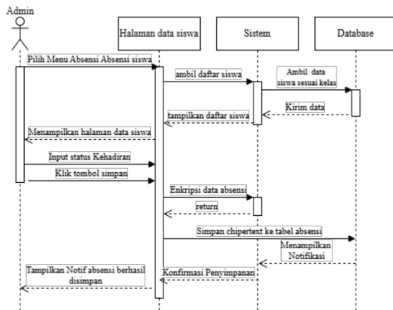
Figure 7. Sequence Diagram for Taking Attendance
