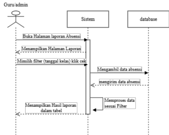
Figure 8. Sequence Diagram of Attendance Report
